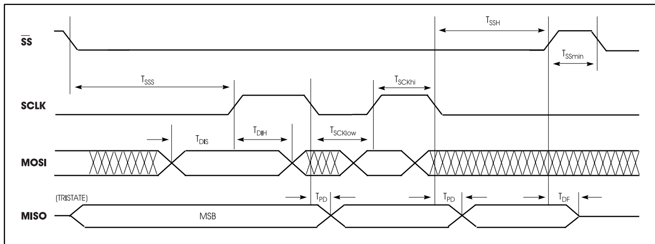
Figure 6: Timing Diagram
