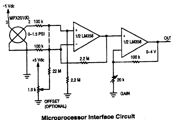
Microprocessor Interface Circuit
