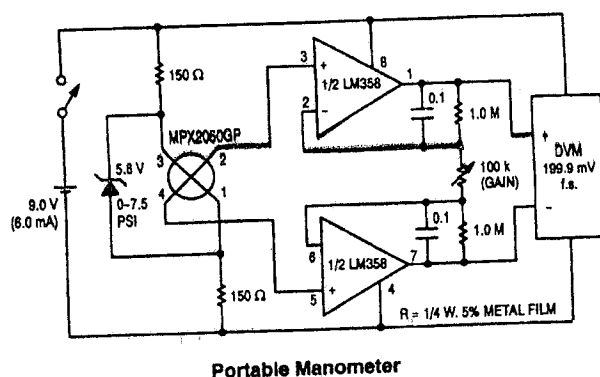
Portable Manometer
