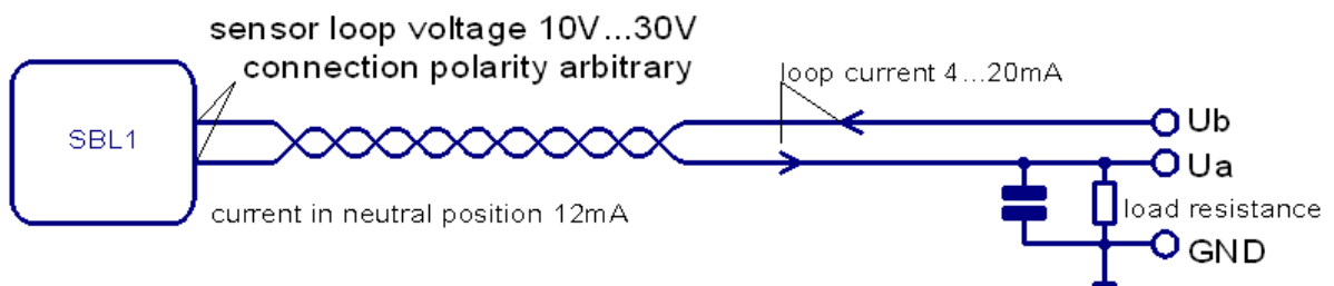
FIGURE 1: Cable Connections
