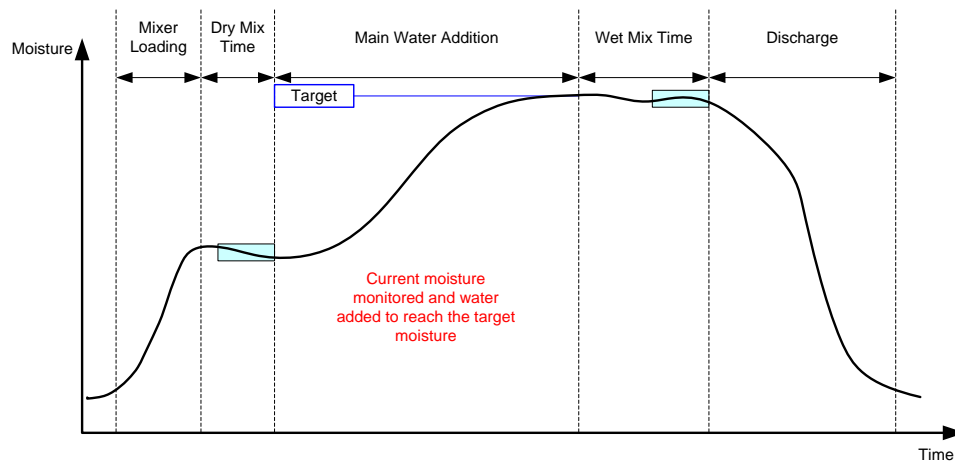
Figure 22: The moisture during AUTO Mode
