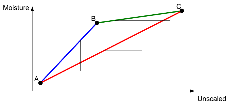
Figure 27: The calibration lines from the 2-step preset mode cycle
