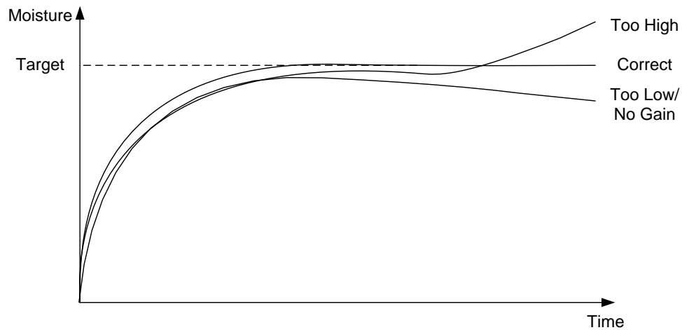
Figure 24: The effect of changing the Integral Gain
