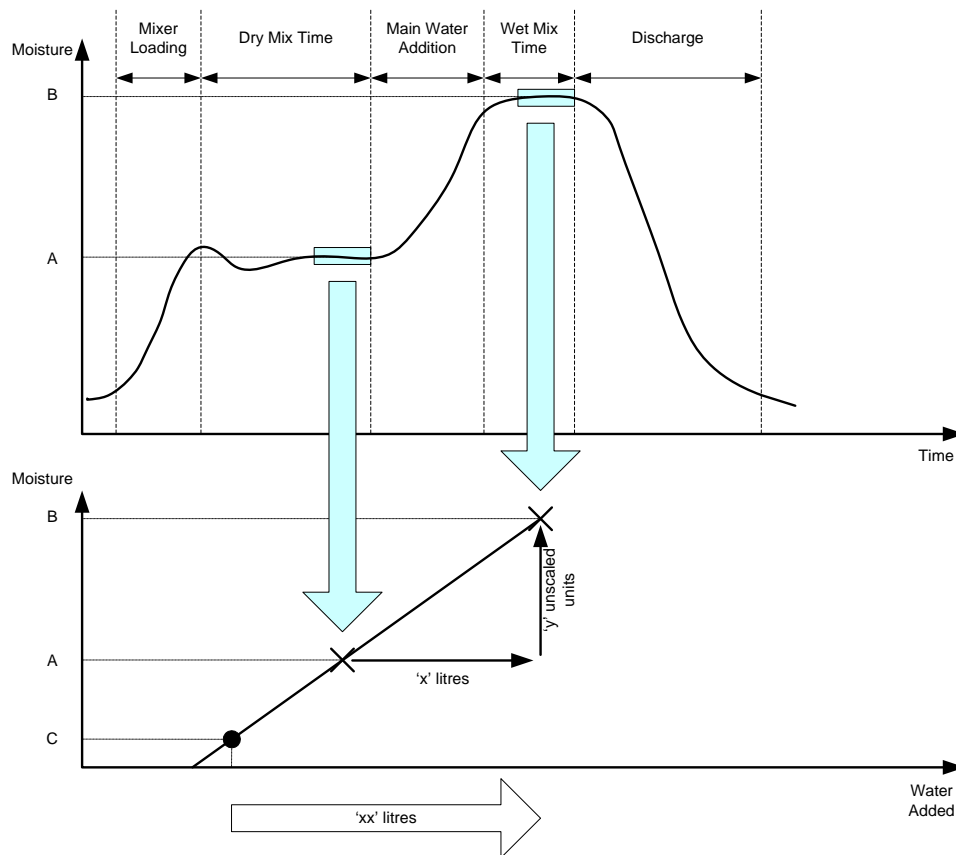
Figure 19: The CALC Mode Calculation
