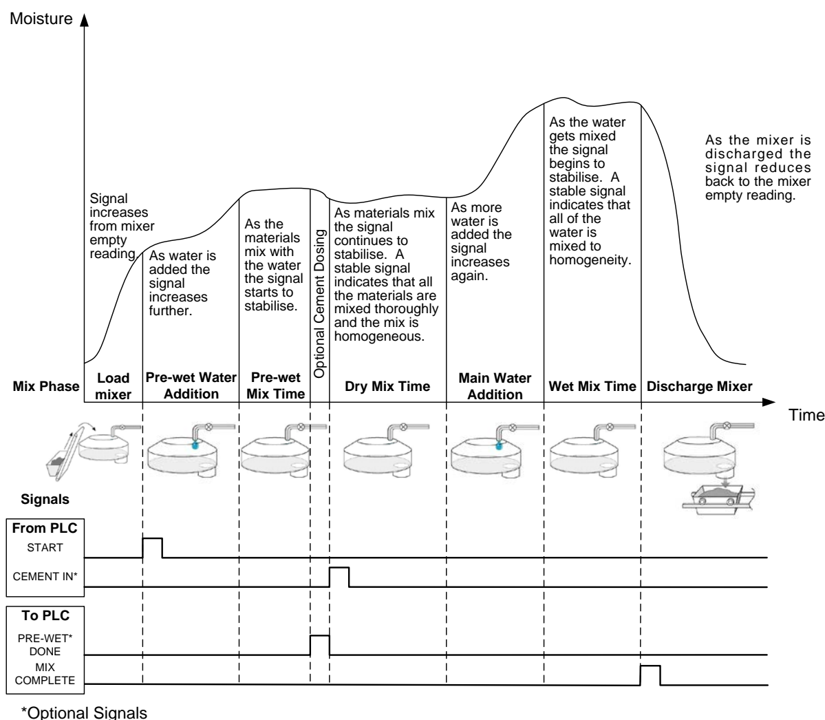
Figure 8: The mix cycle with pre-wet
