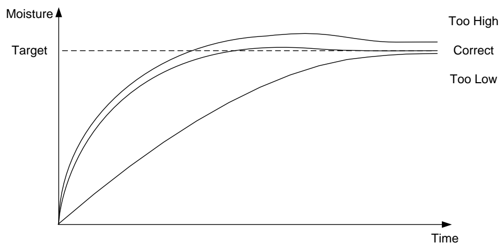
Figure 25: The effect of changing the Derivative Gain
