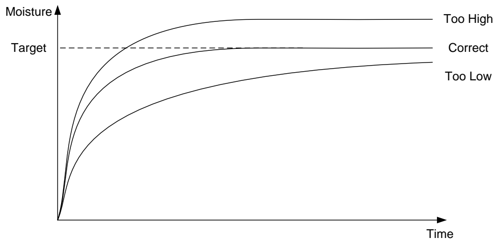
Figure 23: The effect of changing the Proportional Gain
