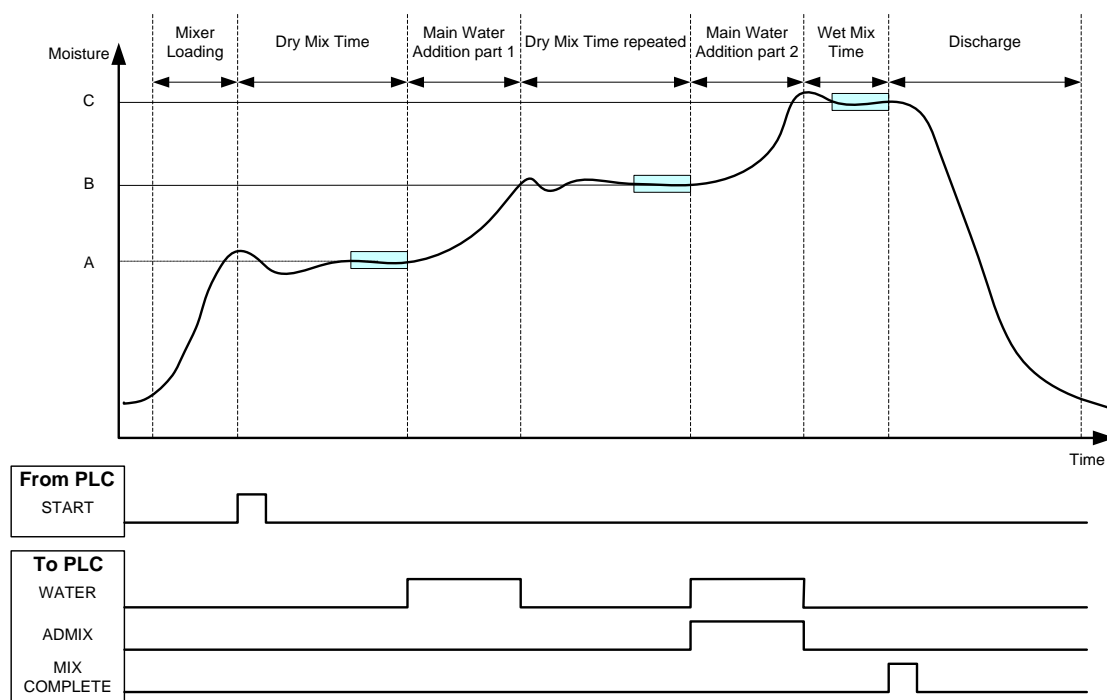
Figure 26: The 2 step preset mode cycle
