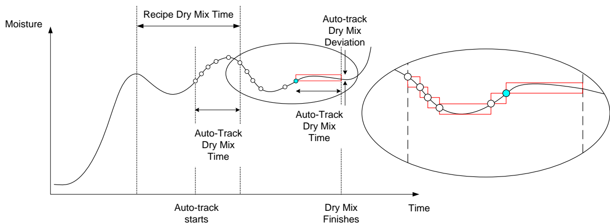
Figure 28: Mix trace showing the Auto-track function
