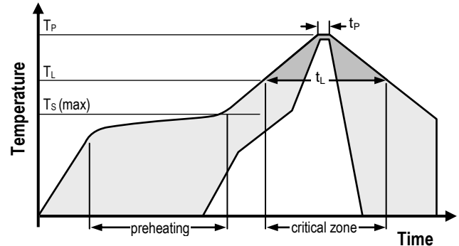
Figure 9 Soldering profile according to JEDEC standard. T_P \leq 260^{\circ}\text{C} and t_P < 30\text{sec} for Pb-free assembly. T_L < 220^{\circ}\text{C} and t_L < 150\text{sec} . Ramp-up/down speeds shall be < 5^{\circ}\text{C}/\text{sec} .
