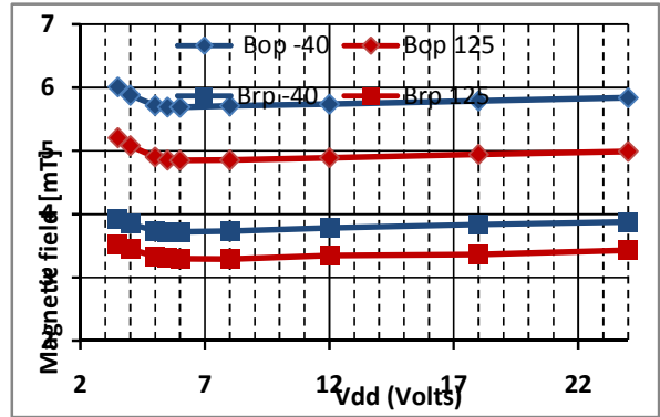
11.2 Magnetic parameters vs. V_{DD}
