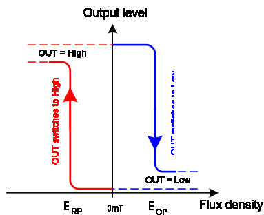
Latch characteristic
