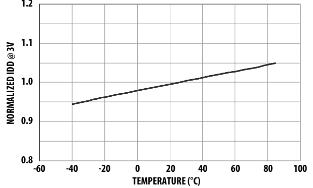
Figure 4b. Normalized IDD vs. Temperature
