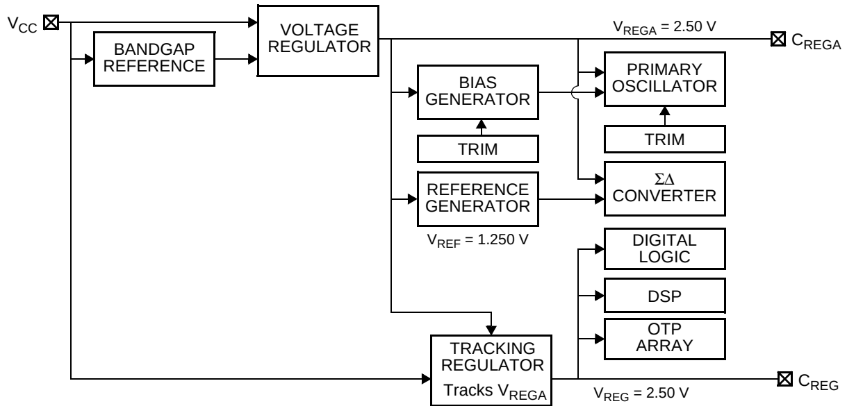
Figure 7. Power Supply
