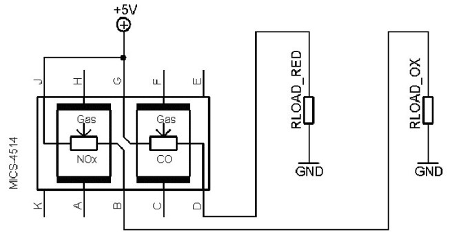
Figure 3: MiCS-4514 with measurement circuit (top view)
