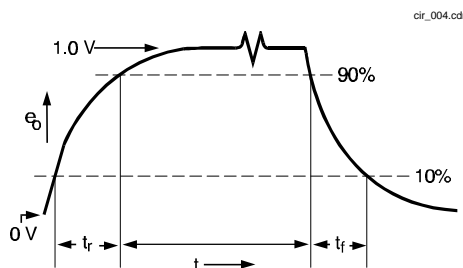
SWITCHING WAVEFORM
