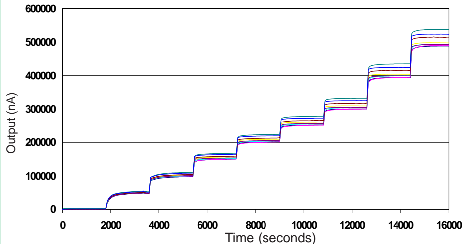
Figure 4 Response to 200ppm HCl
