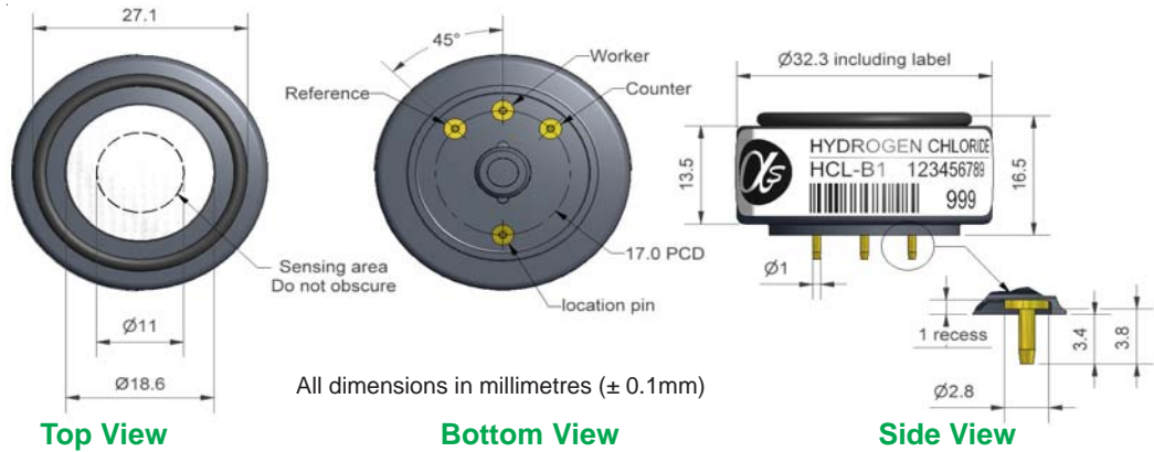
Figure 1 HCL-B1 Schematic Diagram
