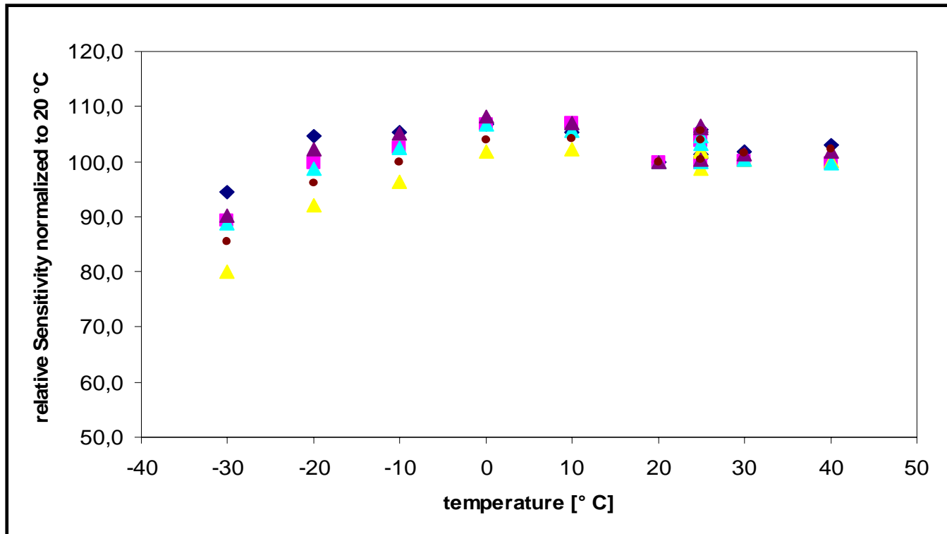
RELATIVE OUTPUT vs. TEMPERATURE: (normalized to the output at 20 °C)
