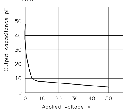
Applied voltage vs. output capacitance Across terminals 5,7 and 6,8 pin Frequency: 1MHz; Ambient temperature: 25°C
