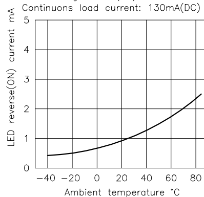
LED reverse(ON) current vs. ambient temperature Load voltage: 400V(DC) Continuous load current: 130mA(DC)
