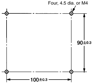
Mounting Holes
