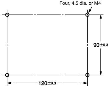
Mounting Holes
