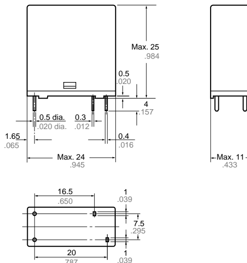
PC board pattern (Copper-side view)
