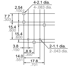
PC board pattern (Copper-side view)
