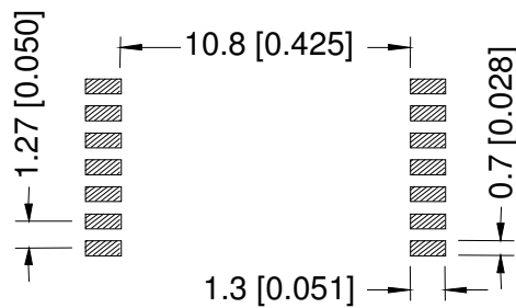
Fig. 9: Recommended pad-layout for MS5536-60CPJU
