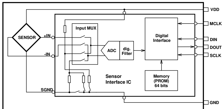
Fig. 1: Block Diagram MS5536-60C
