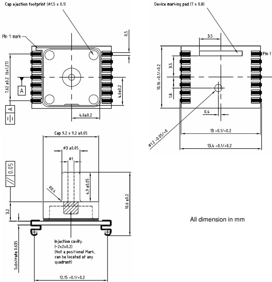
Fig. 8: Device package outlines of MS5536-60CPJU
