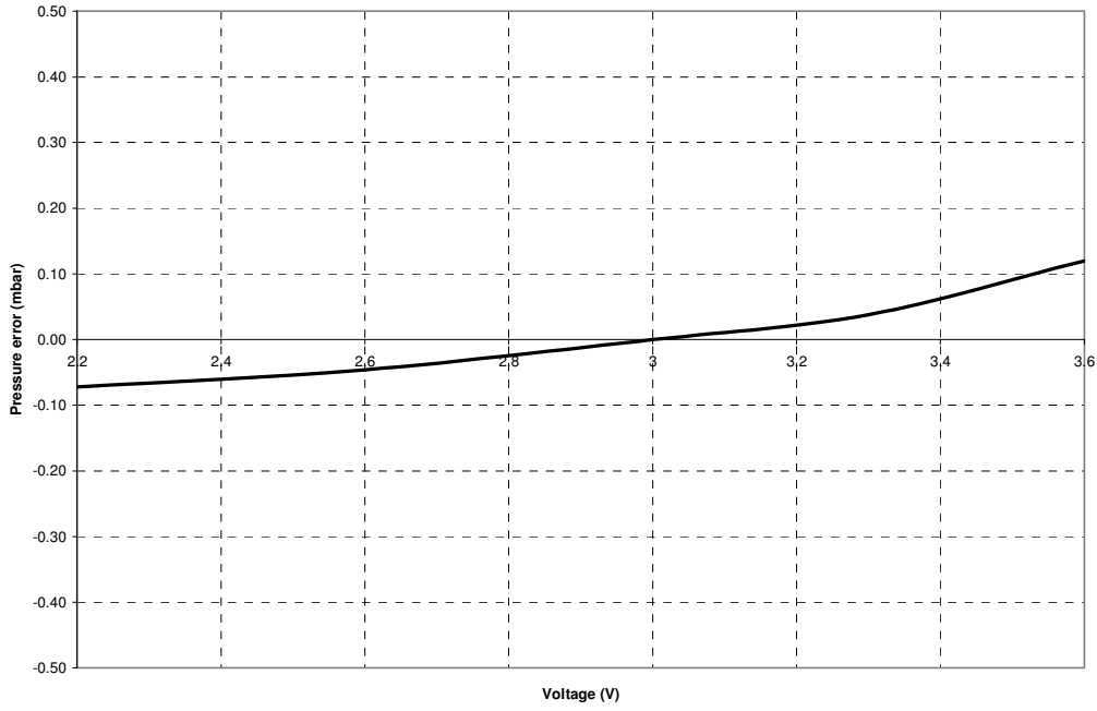
Pressure error vs supply voltage (typical)
