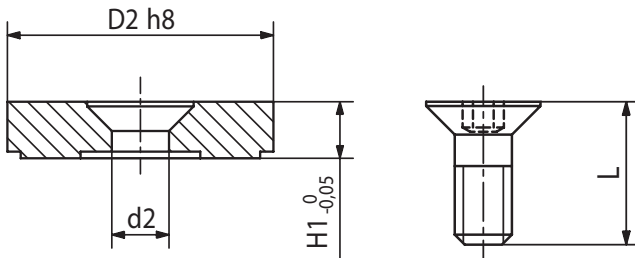
Fig. 4: One countersunk screw is delivered with each preloading disk.
