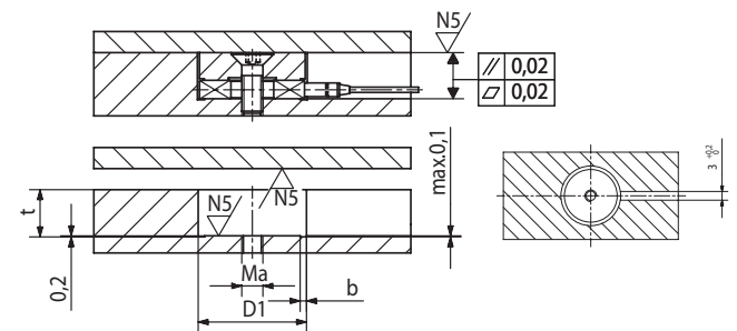
Fig. 3: Shunt mounting with preloading disk
