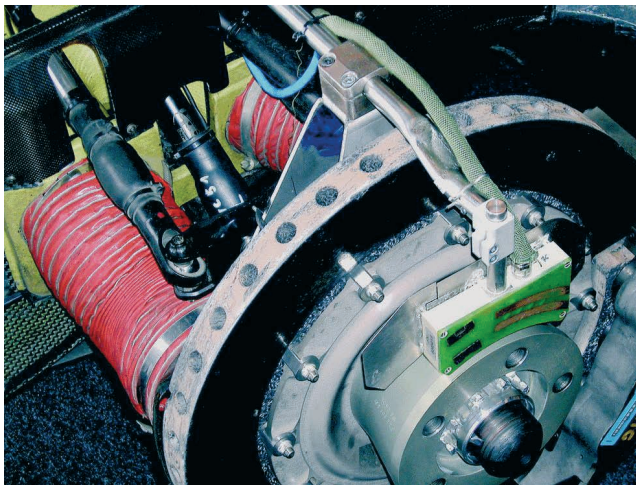
Fig. 2: Stator mounted on vehicle
