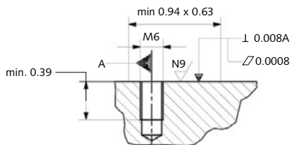
Mounting AE-Sensor
