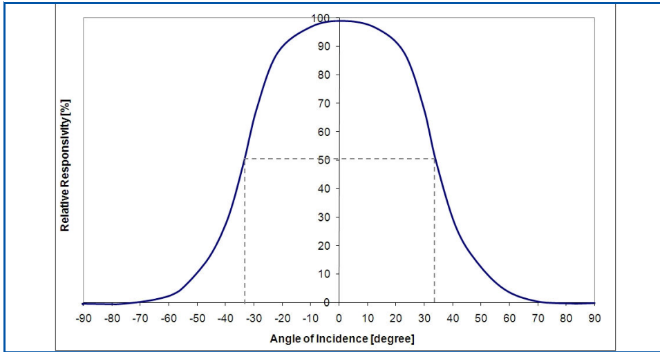
Figure 1 Field of View Curve
