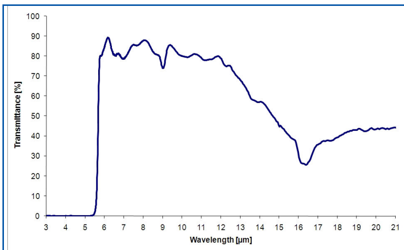
Figure 2 Typical filter transmission curve
