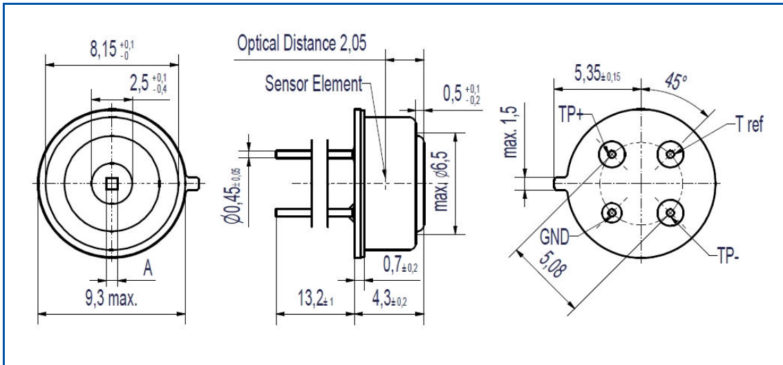
Figure 3 Mechanical Drawing of the TPD 1T 0224 (Drawing No.: 2/71829-0)
