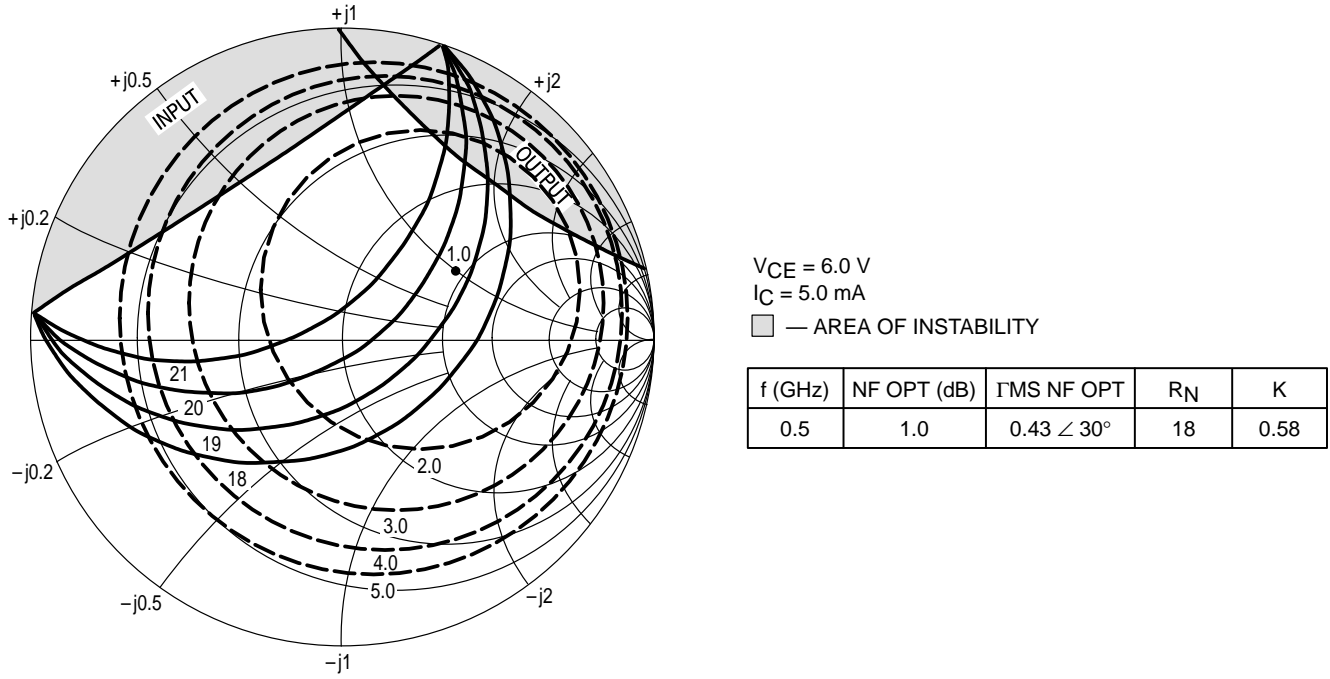
Figure 19. MMBR941LT1, T3 Constant Gain and Noise Figure Contours (f = 0.5 GHz)
