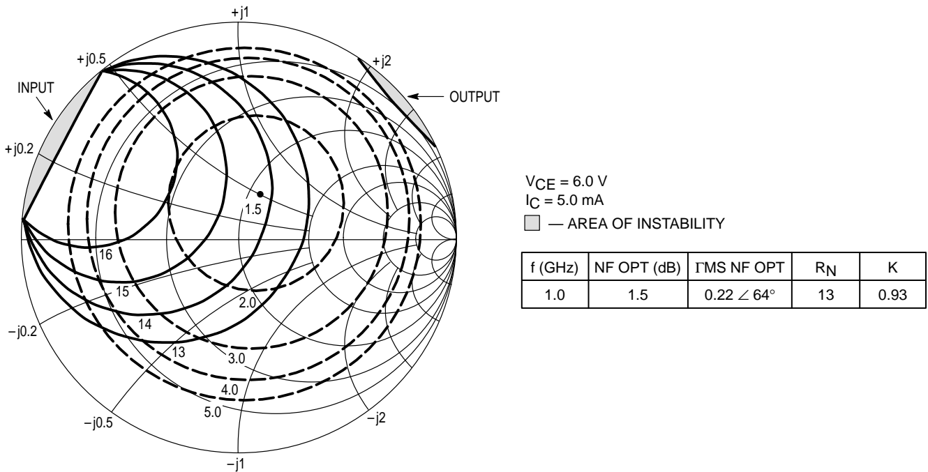
Figure 20. MMBR941LT1, T3 Constant Gain and Noise Figure Contours (f = 1.0 GHz)
