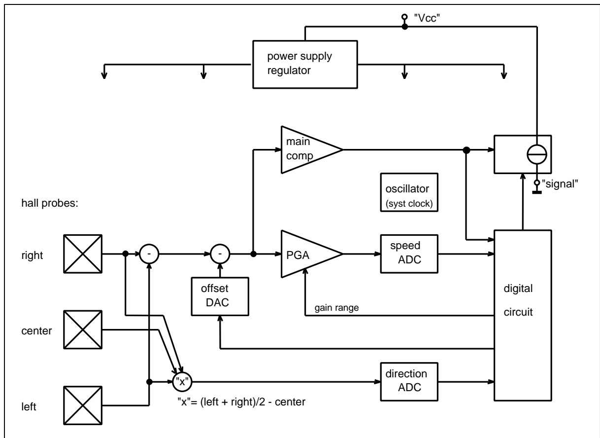
Figure 2 Block diagram
