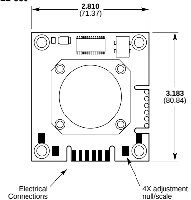
AccuSwitch w/Standoffs P/N 02118111-000
