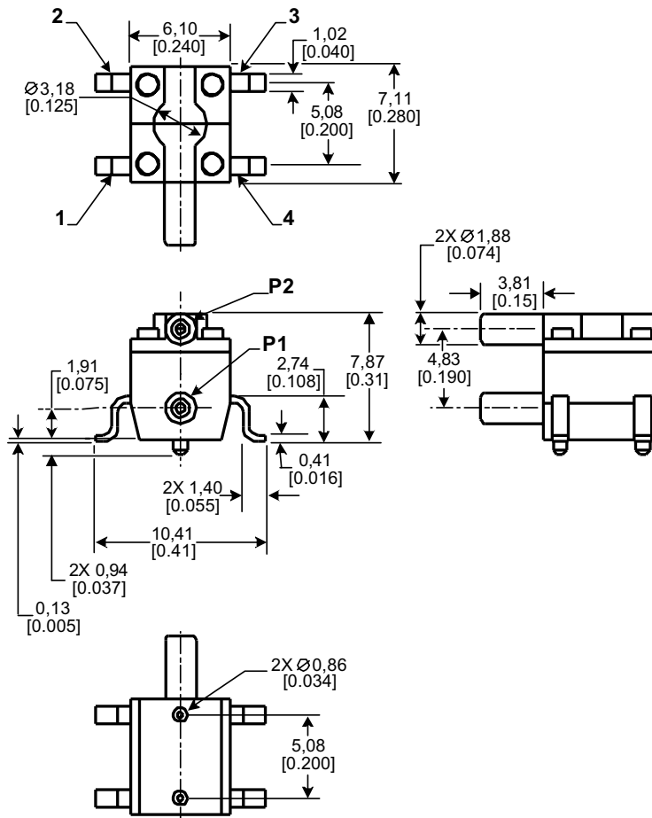
MOUNTING DIMENSIONS mm[in] (for reference only)
