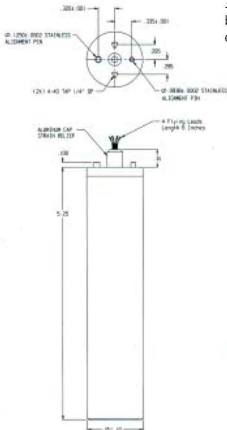
Outline Drawing (CHS110TB shown)
