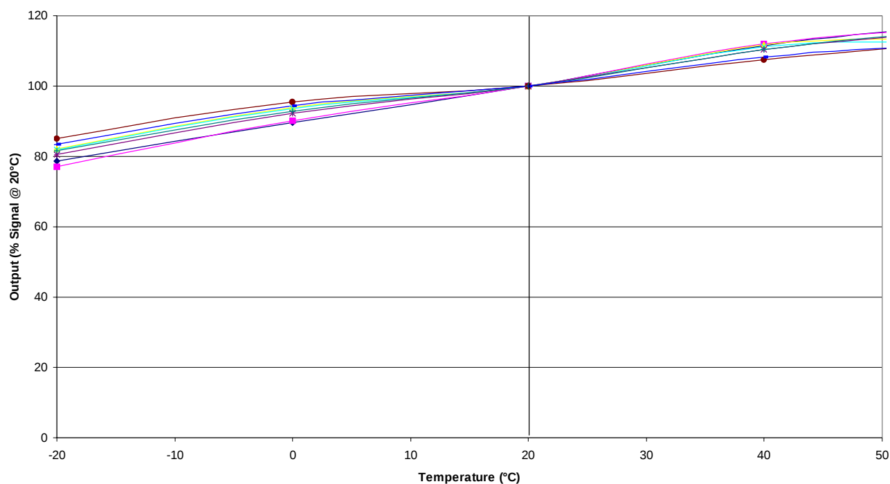
42HS-2 Hydrogen Sulphide CiTiceL - Output vs Temperature
