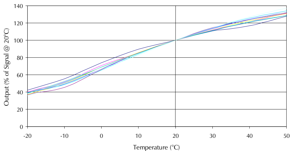
7ETO Ethylene oxide CiTiceL - Output vs Temperature
