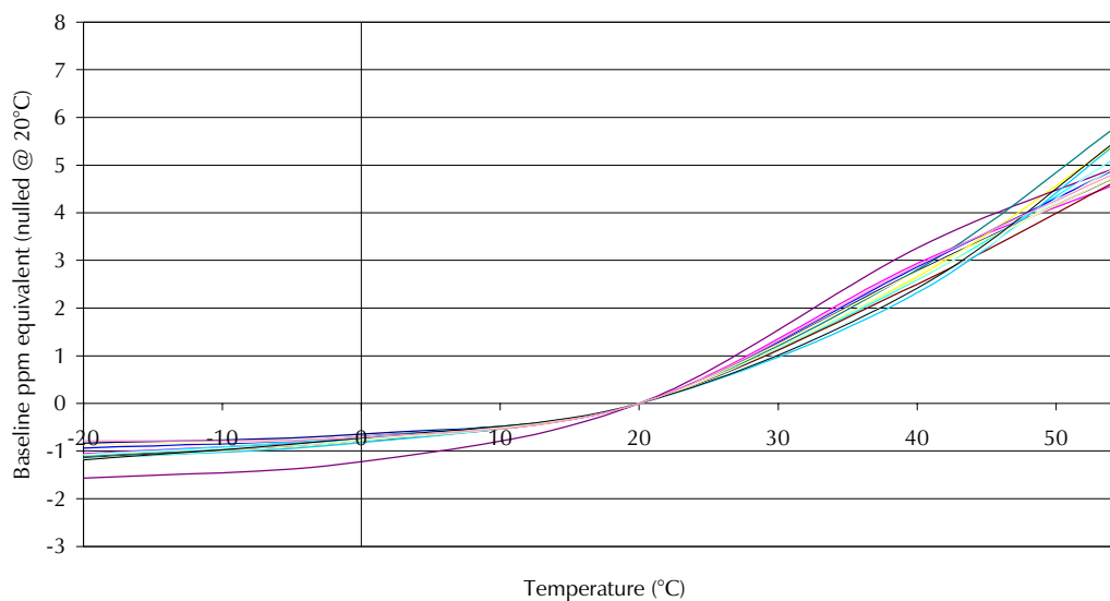
4ETO Ethylene Oxide CiTiceL - Baseline vs Temperature
