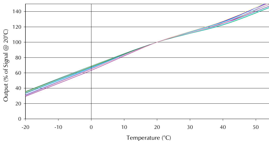
4ETO Ethylene Oxide CiTiceL - Output vs Temperature
