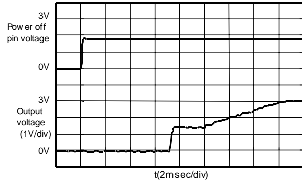
S-8520/1C30MC (Vin:9.0V)
