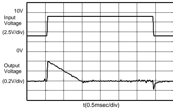
S-8520/1A30MC
