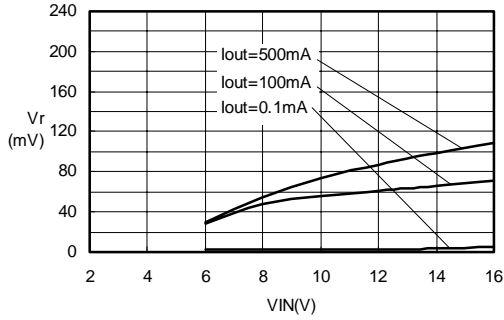
Ripple voltage-VIN S-8520F50MC(Cout:22uF)
