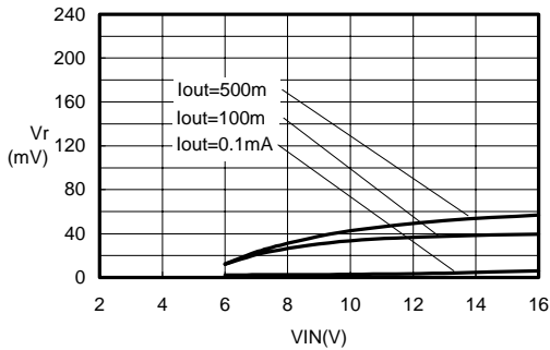
Ripple voltage-VIN S-8520B50MC(Cout:22uFx2)
