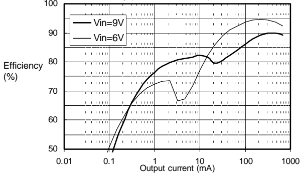
S-8521F50MC Output current - Efficiency (D62F/22uH, TM6201)
