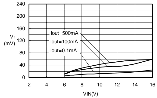
Ripple voltage-VIN S-8521B50MC(Cout:22uFx2)
