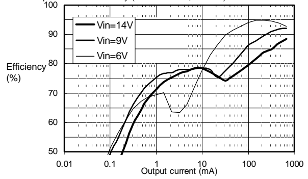
S-8521F50MC Output current - Efficiency (CDH113/22uH, IRF7606)
