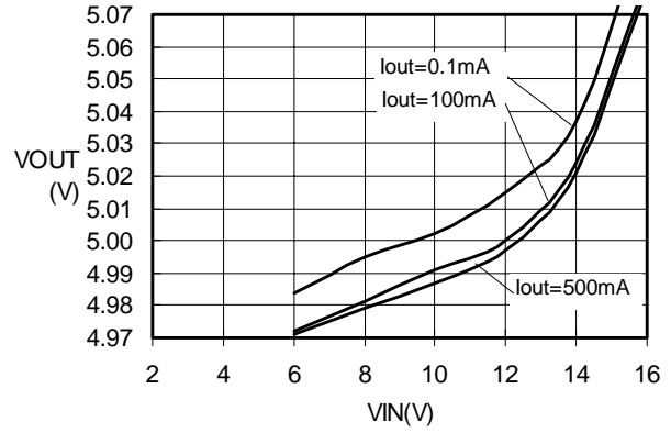
VOUT-VIN S-8521F50MC (Ta=25°C)
