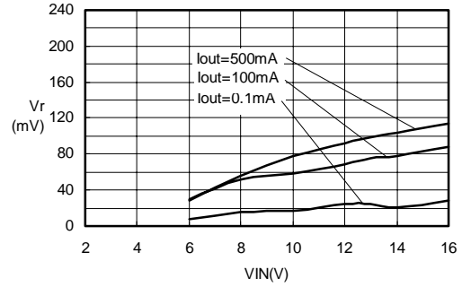
Ripple voltage-VIN S-8521F50MC(Cout:22uF)
