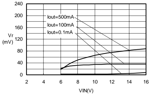
Ripple voltage-VIN S-8520D50MC(Cout:47uFx2)
