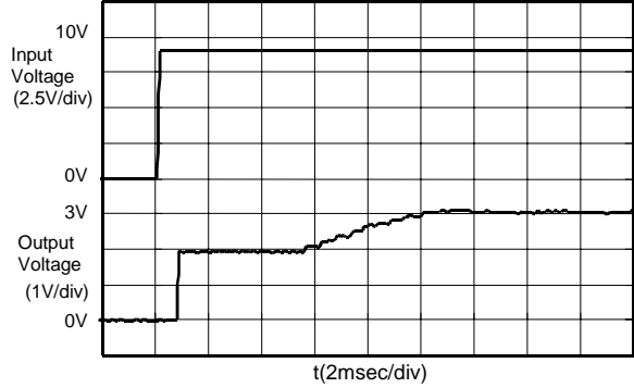
S-8520/1C30MC (Vin:0→9.0V)
