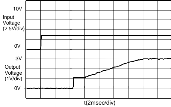
S-8520/1C30MC (Vin:0→3.6V)
