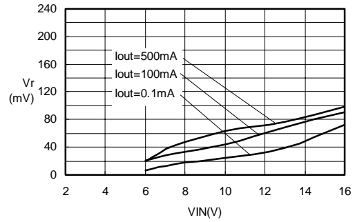
Ripple voltage-VIN S-8521D50MC(Cout:47uFx2)
