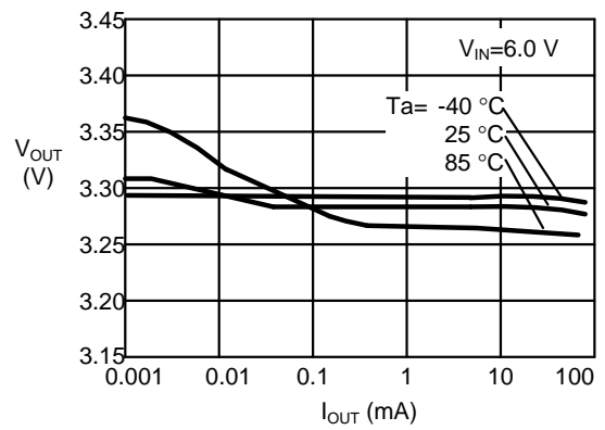
1.6 Output current ( I_{OUT} )-Output voltage ( V_{OUT} )
