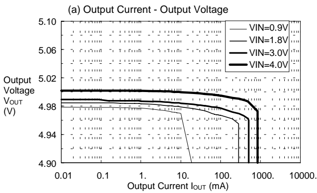
(24)S-8327B50(CD54:47 \mu H,Rb=1k \Omega ,Cb=0.0022 \mu F)
