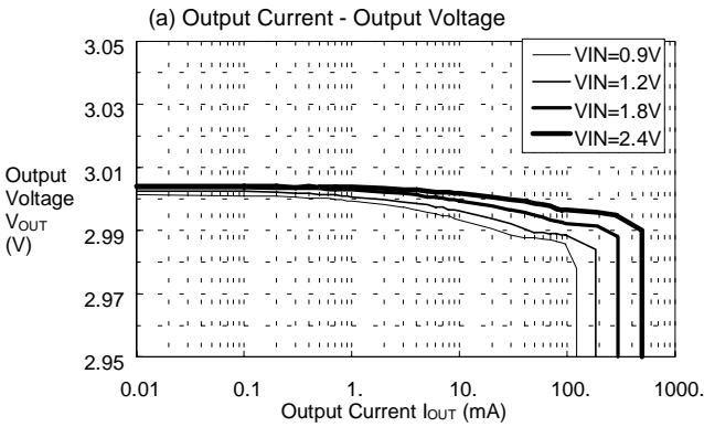
(20)S-8327B30(CD54:47 \mu H,Rb=1k \Omega ,Cb=0.0022 \mu F)
