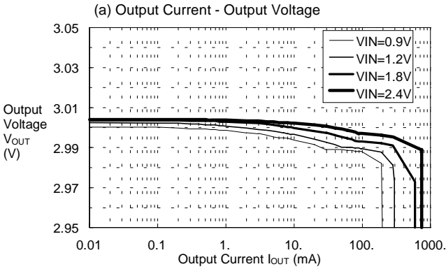
(19)S-8327B30(CD105:22 \mu H,Rb=1k \Omega ,Cb=0.0022 \mu F)
