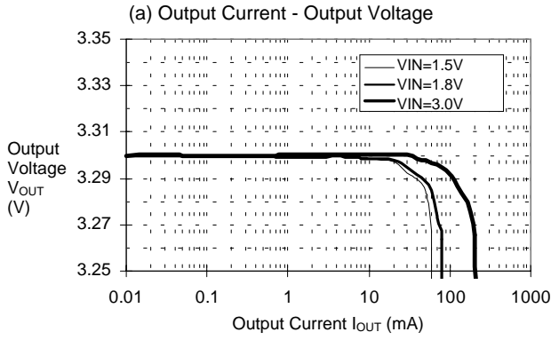
(14)S-8323H33(D62F:22μH)
