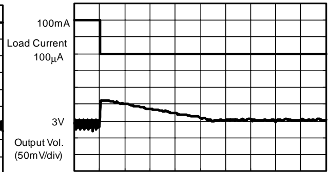
t (5msec/div)
