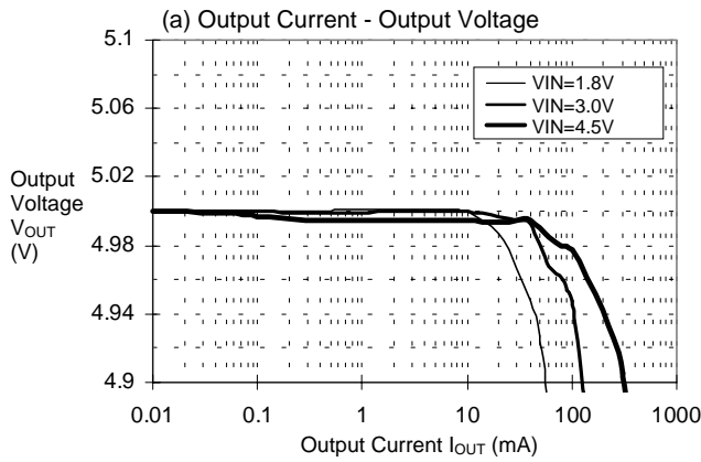
(15)S-8323H50(CDRH 4D18:22μH)
