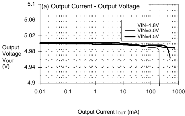
(29)S-8327H50(CDH113:10μH)
