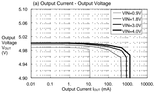
(23)S-8327B50(CD105:22 \mu H,Rb=1k \Omega ,Cb=0.0022 \mu F)
