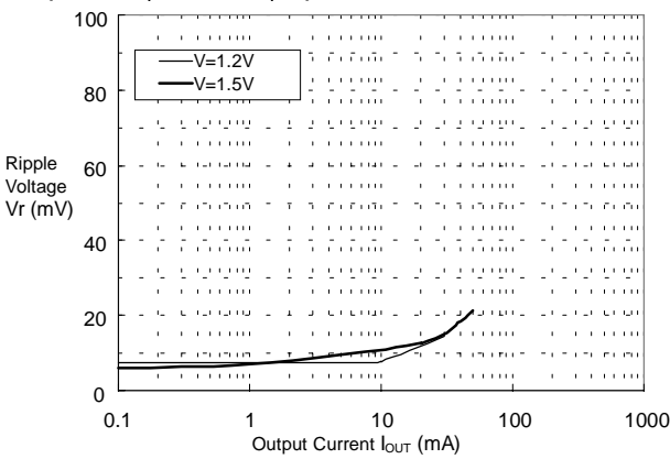
(17)S-8323H50 (D62F:22 \mu H,C OUT :22 \mu F )
