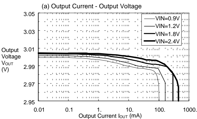
(21)S-8327B30(D75C:47 \mu H,Rb=1k \Omega ,Cb=0.0022 \mu F)
