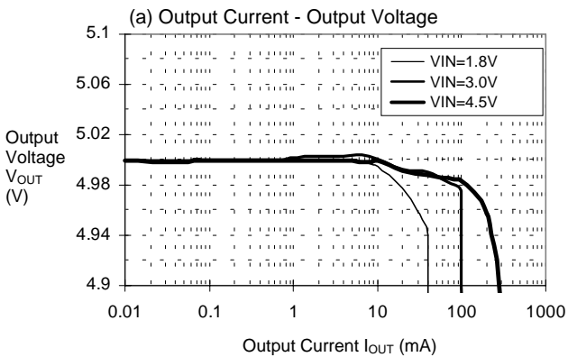
(17)S-8323H50(D62F:22μH )
