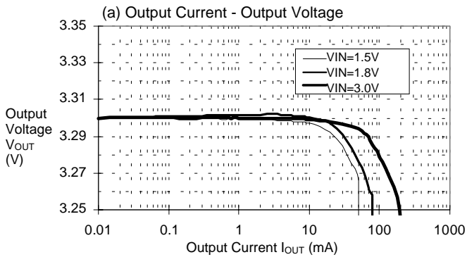
(13)S-8323H33(D62F:10μH)
