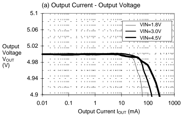
(17)S-8323H50(D62F:22μH )
