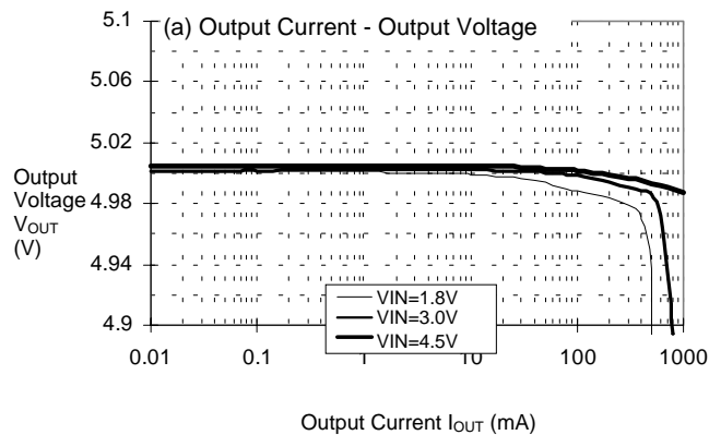
(29)S-8327H50(CDH113:10μH)
