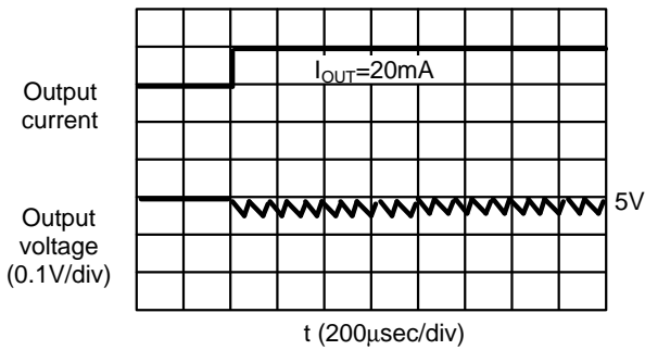
S-8322AA V_{IN}=3\text{ V} , I_{OUT}=10\mu\text{A}\rightarrow 20\text{mA}
