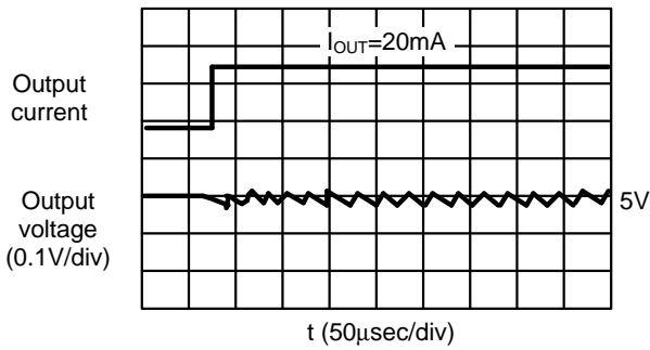
S-8321AA V_{IN}=3\text{ V} , I_{OUT}=10\mu\text{A}\rightarrow 20\text{mA}
