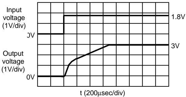
S-8321AI V_{IN} = 0 1.8 V, R_L = 250\Omega
