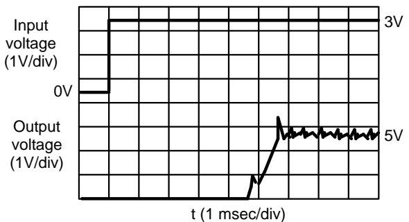
S-8322AA V_{IN} = 0 3 V, R_L = 250\Omega
