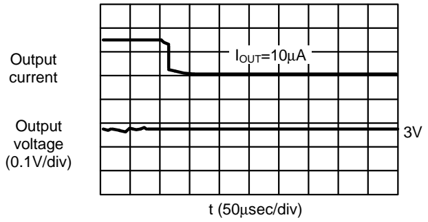
S-8321AA V_{IN}=3\text{ V} , I_{OUT}=20\text{mA}\rightarrow 10\mu\text{A}
