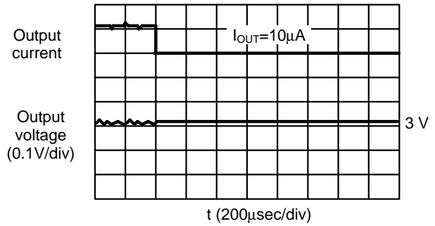
S-8322AA V_{IN}=3\text{ V} , I_{OUT}=20\text{mA}\rightarrow 10\mu\text{A}
