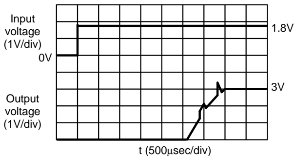
S-8322AI V_{IN} = 0 1.8 V, R_L = 250\Omega
