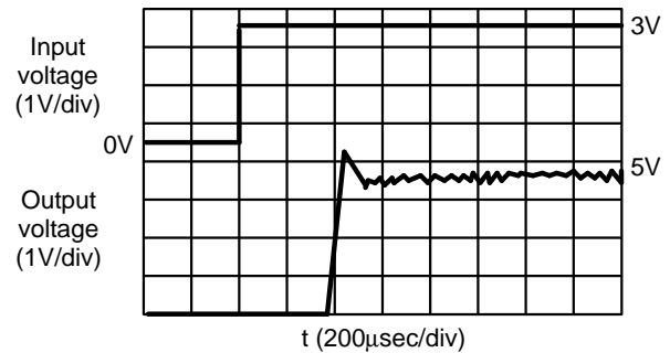
S-8321AA V_{IN} = 0 3 V, R_L = 250\Omega
