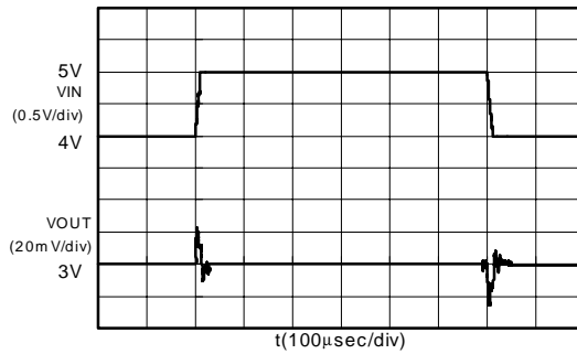
S-816A30AMC (Iout:300mA)
