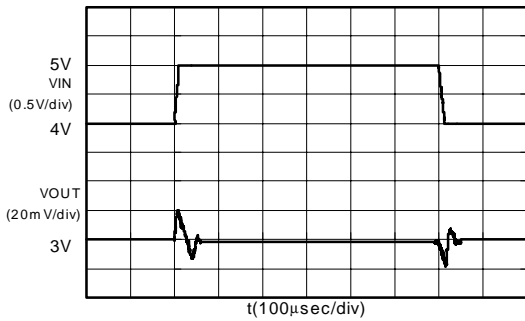
S-816A30AMC (Iout:10mA)
