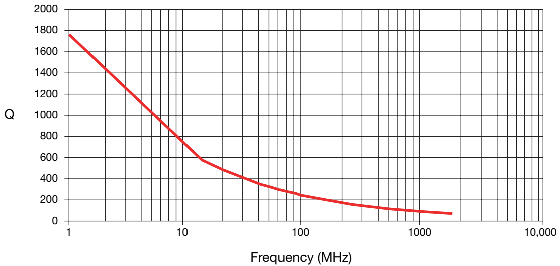
22pF Q vs. Frequency
