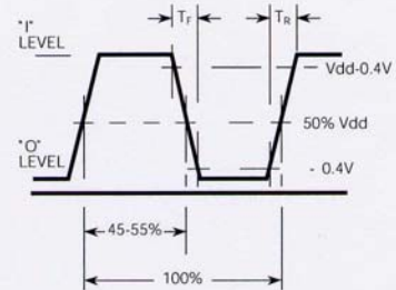
Fig. 3. Timing
