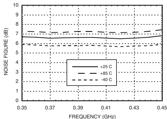
Noise Figure vs. Temperature @ 400 MHz
