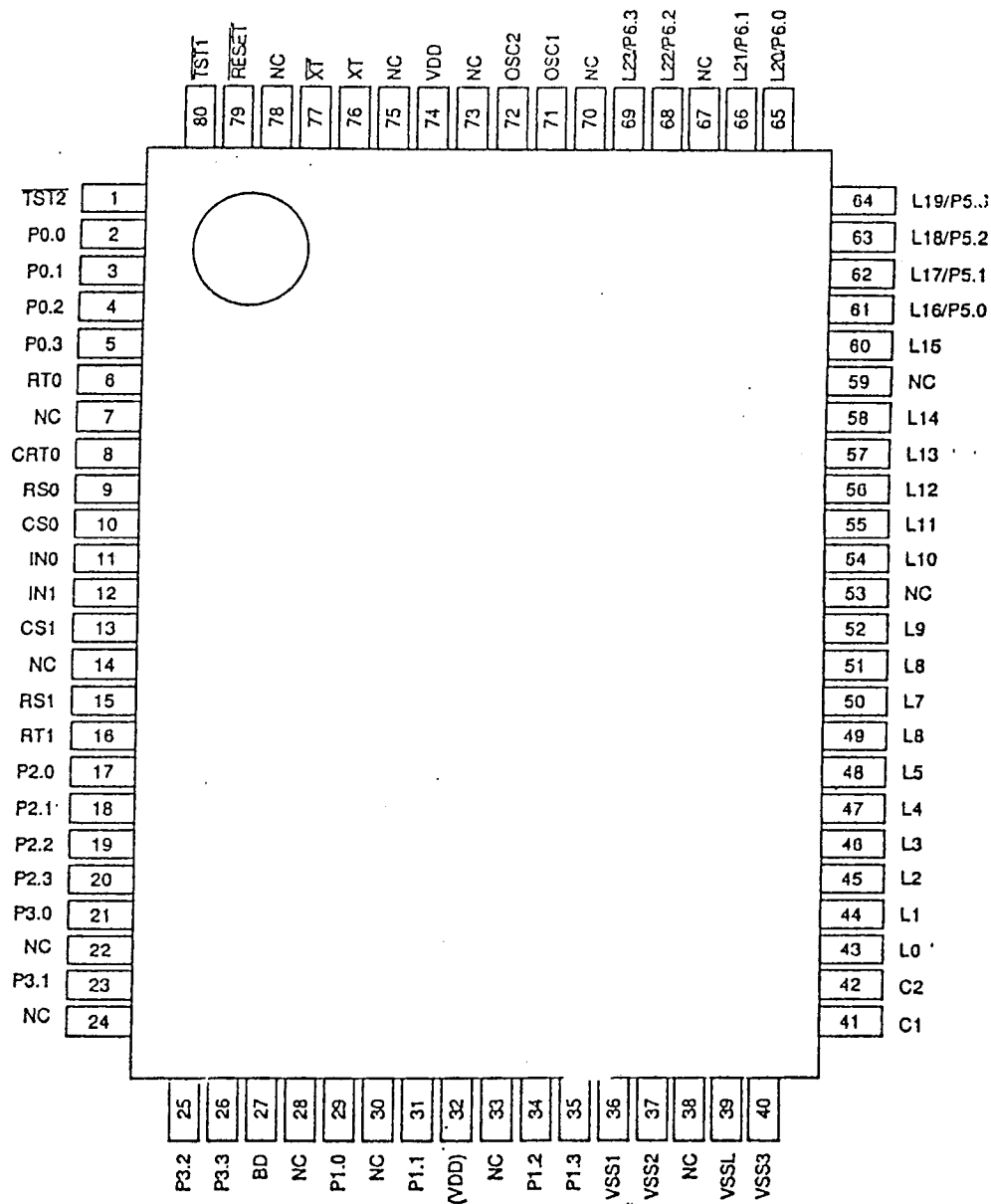
Figure 3.1 Pin layout of the SS0202 GS-K-F
