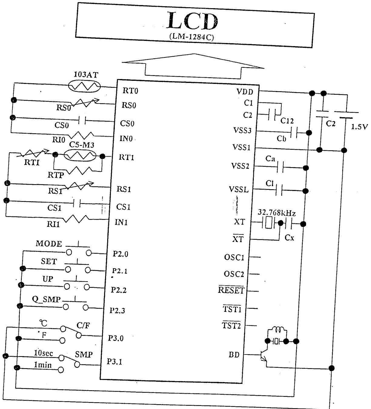
Figure 5.1 Reference circuit diagram of the SS0202 Circuit
