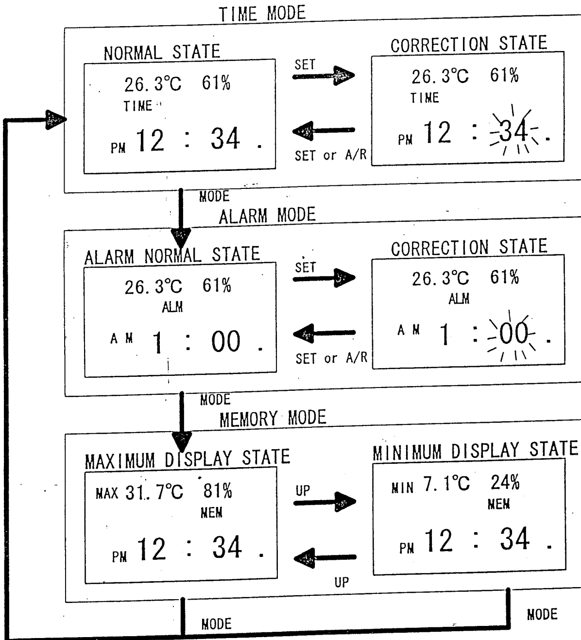
Figure 8.1 Mode Transition Diagram of the SS0202
