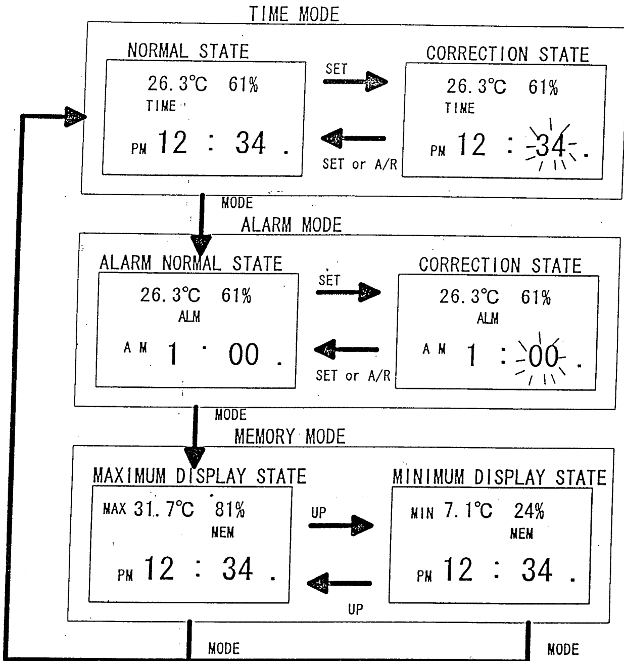
Figure 8.1 Mode Transition Diagram of the SS0202
