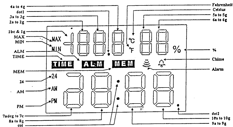
Figure 4.2 LCD Element name
