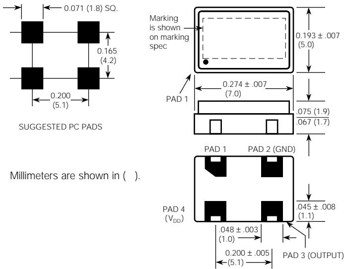
"T" Package
