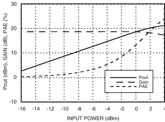
Power Compression @ 2100 MHz [1]
