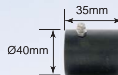
Standard Mounting Collar
