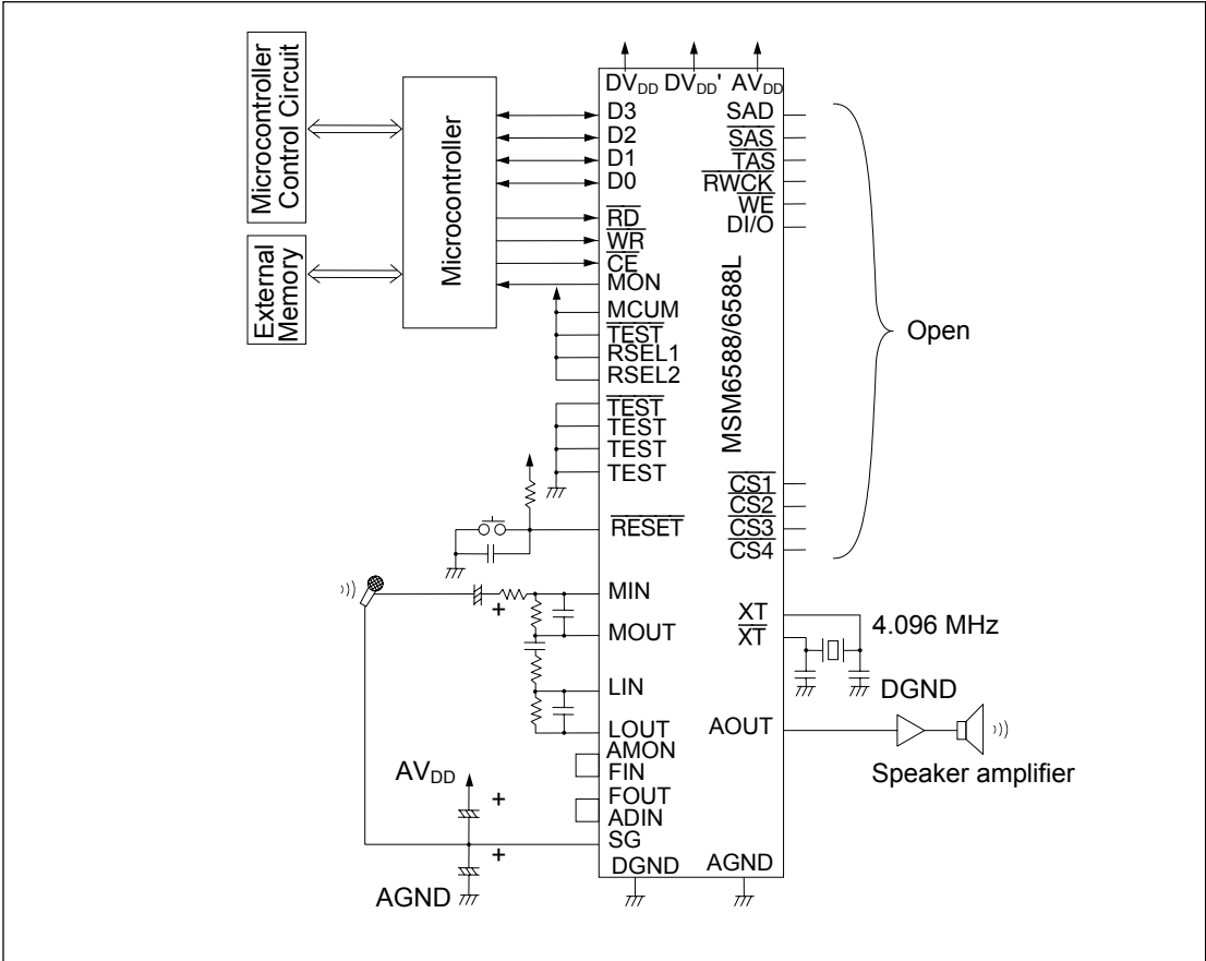
Figure 3 Example of Application Circuit When Record/Playback is Made Using EXT Command
