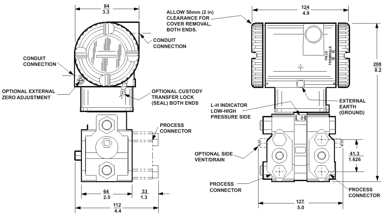
TRADITIONAL STRUCTURE DIMENSIONS (NOMINAL) \frac{\text{mm}}{\text{in}}
