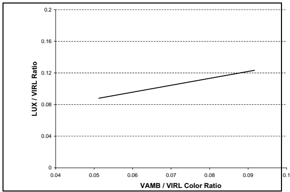
Figure 15. Lux/VIREL Ratio vs. Color Ratio
