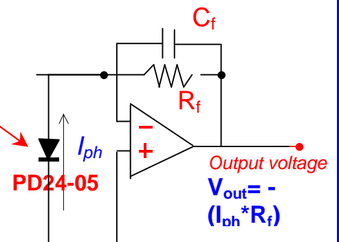
Basic Circuit Connections
