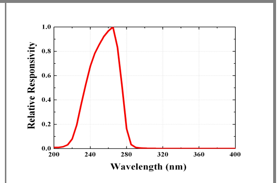
Fig. 2 Responsivity Curve
