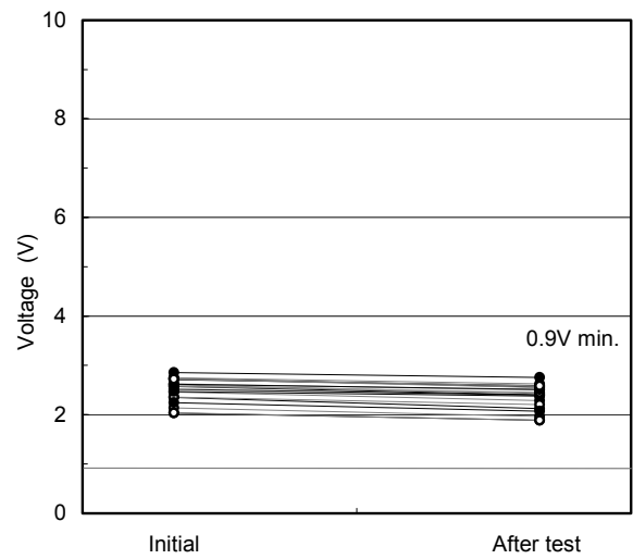
Release voltage
