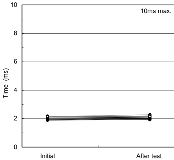
Operate time
