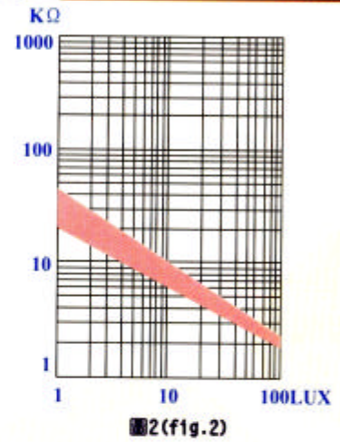
Illuminance-resistance characteristic
