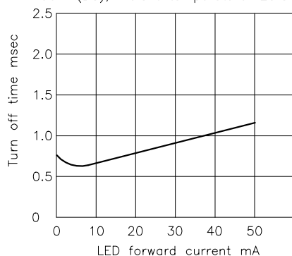
LED forward current vs. turn off time Across terminals 5,7 and 6,8 pin; Load voltage: 350V(DC); Continuous load current: 130mA(DC); Ambient temperature: 25°C
